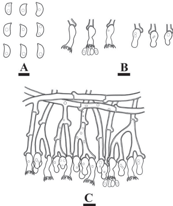
Figure 4. Microscopic structures of Burgella albofarinacea (holotype): basidiospores (A), basidia and basidioles (B), a section of hymenium (C). Scale bars: 5 µm (A); 10 µm (B, C).
