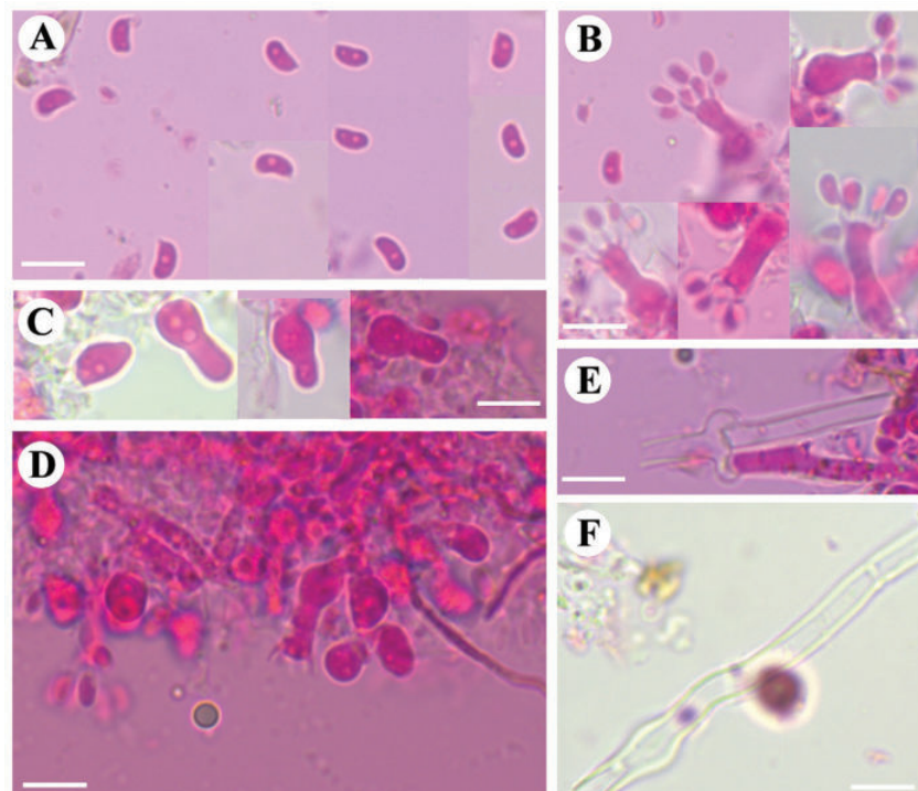
Figure 5. Microscopic structures of Burgella albofarinacea (holotype): basidiospores (A), basidia (B), basidioles (C), a section of hymenium (D), generative hyphae (E, F). Scale bars: 10 µm (A–F).
