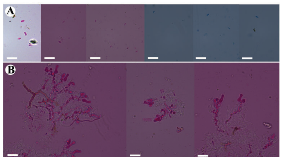
Figure 17. Microscopic structures of Sistotrema sinense (holotype): basidiospores (A), a section of hymenium (B). Scale bars: 10 \mu m (A, B).
